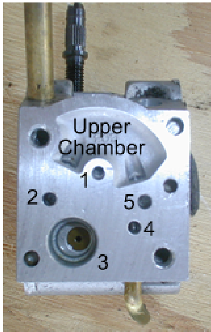
Figure 7. WT363 top of carburetor body.
