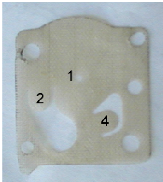
Figure 8. Carburetor body check valve wafer.
