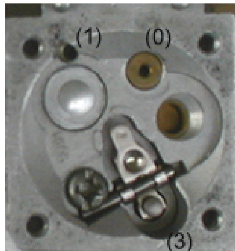
Figure 9. WA363 Lower chamber with diaphragm removed.
