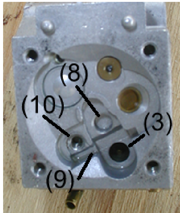
Figure 15. Fuel flow parts removed. by Lynn W. Graves
