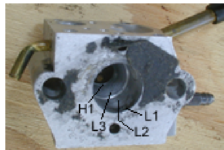
Figure 12. WT363 Venturi view of fuel metering ports.
