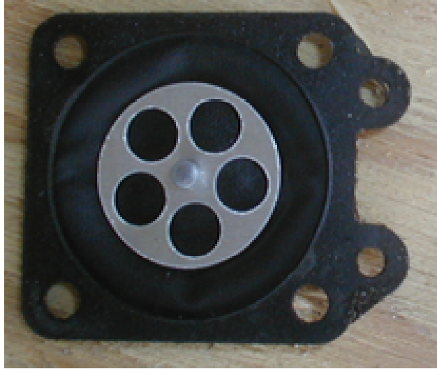
Figure 13. WRONG DEAL, thick gasket should be behind the diaphragm.
