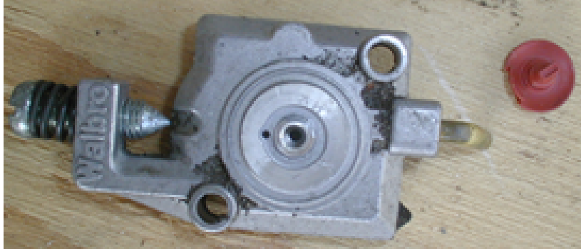
Figure 5. WT363 top plate with check valve removed.
