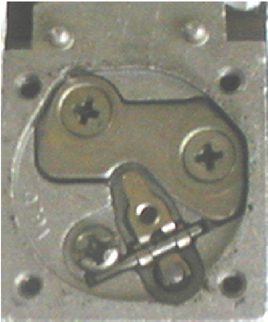
Figure 10. WA229 Lower chamber with diaphragm removed.
