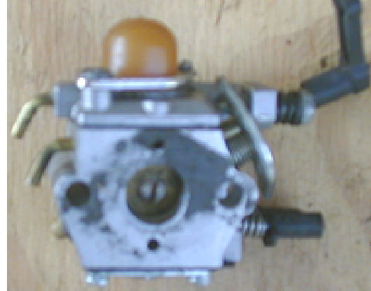
Figure 3. WT363 viewed from engine side.
